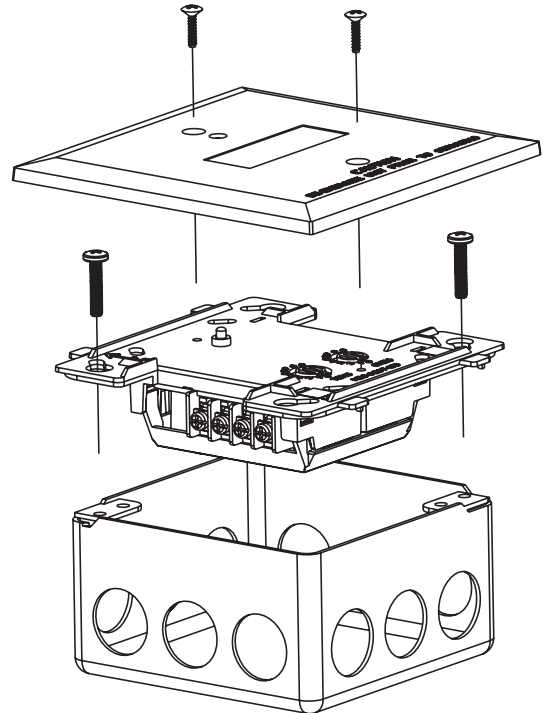
FIGURE 2. MODULE MOUNTING:
