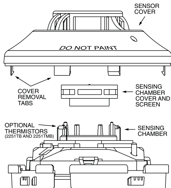
FIGURE 4. SENSOR ASSEMBLY:
