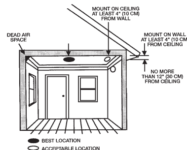
Figure 5: RECOMMENDED SMOKE ALARM MOUNTING LOCATIONS.
