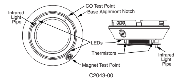
FIGURE 4. CLEANING THE FIRE/CO DETECTOR
