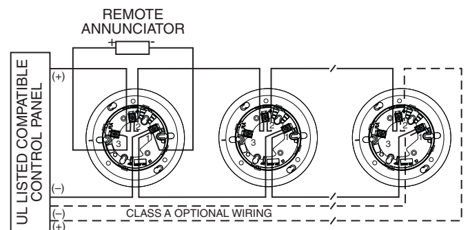
FIGURE 1. WIRING DIAGRAM
