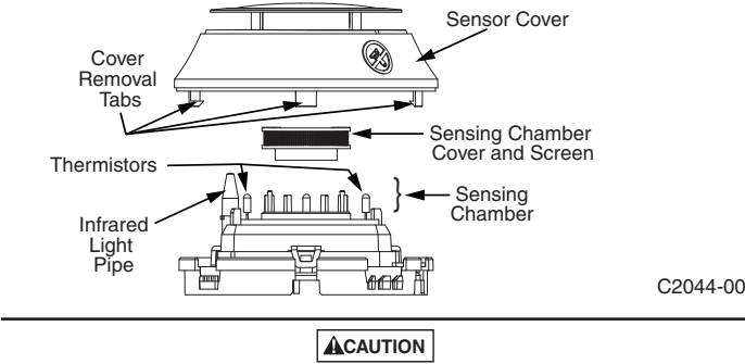
FIGURE 4. CLEANING THE FIRE/CO DETECTOR
