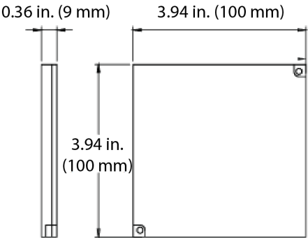
Figure 3: Reflector
