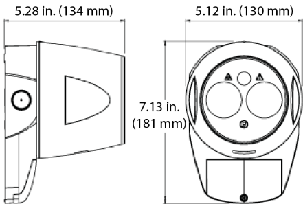
Figure 2: Fireray One
